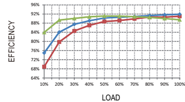
RSD-60H-24
