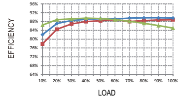
RSD-60H-3.3
